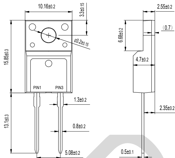
TO-220FAC Dimensions in millimeters
