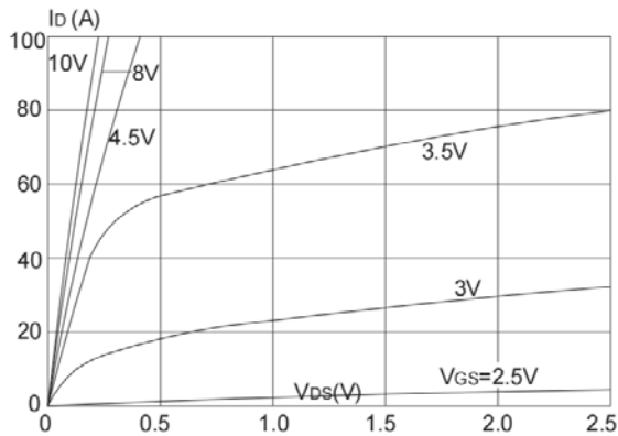
Figure1: Output Characteristics
