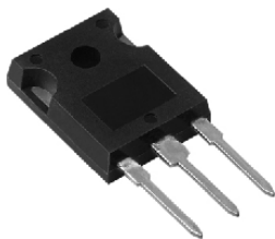
TO-247 MURE7560PT
