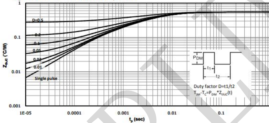
Fig 12: Max. Transient Thermal Impedance
