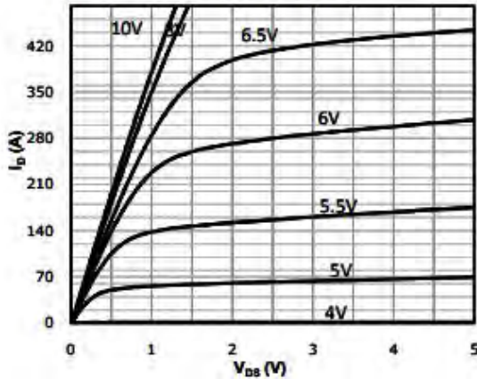
Fig 1: Output Characteristics
