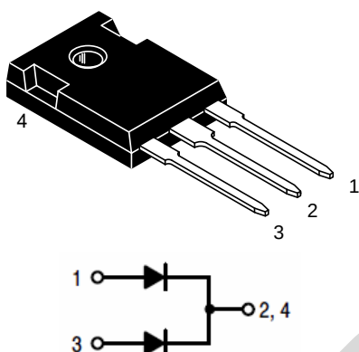
TO-247 MURE6020PT
