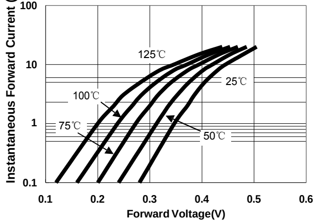
Typical Forward Voltage Characteristics
