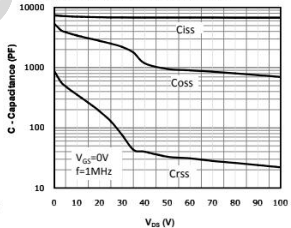
Fig 6: Capacitance Characteristics
