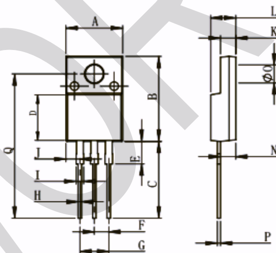
TO-220F
