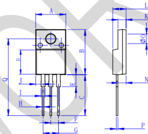
TO-220F
