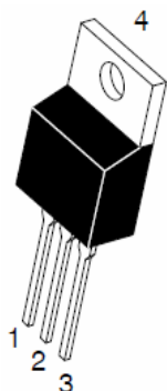
MUR1040CT TO-220AB
