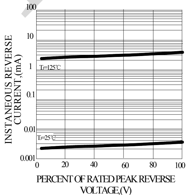
FIG.4-TYPICAL REVERSE CHARACTERISTICS
