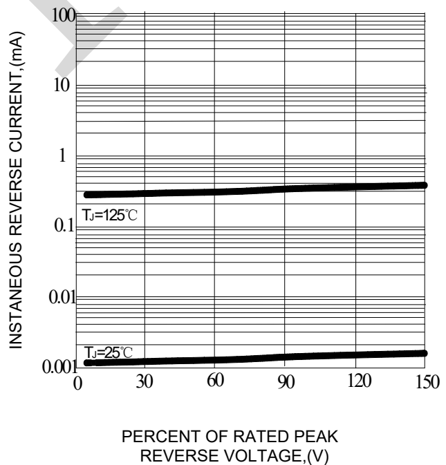
FIG.4-TYPICAL REVERSE CHARACTERISTICS
