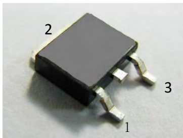
MBR20100D TO-252
