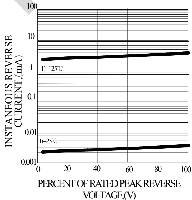
FIG.4-TYPICAL REVERSE CHARACTERISTICS
